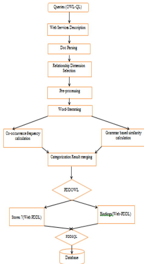
Fig 6: Integrating databases into semantic Web
