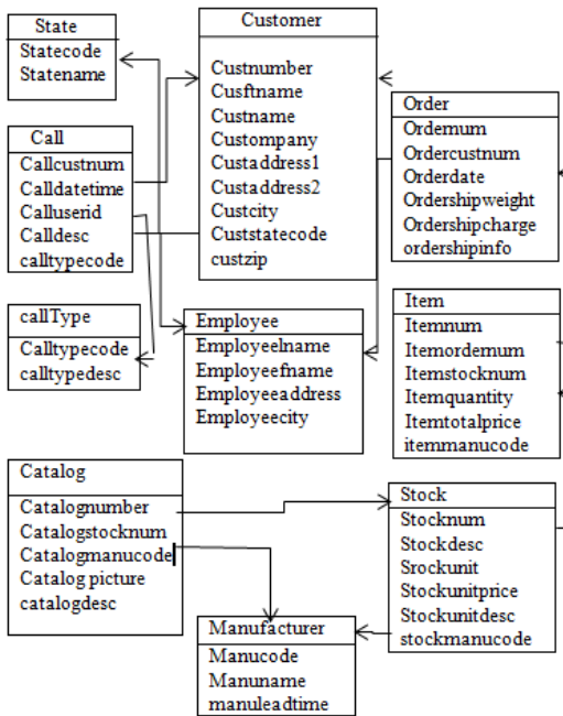
Figure 1. The database schema of Stores7
