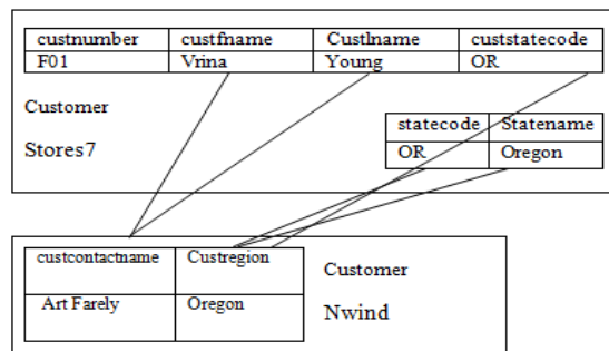
Figure.4 Portions of two database schemas and the mapping between them
